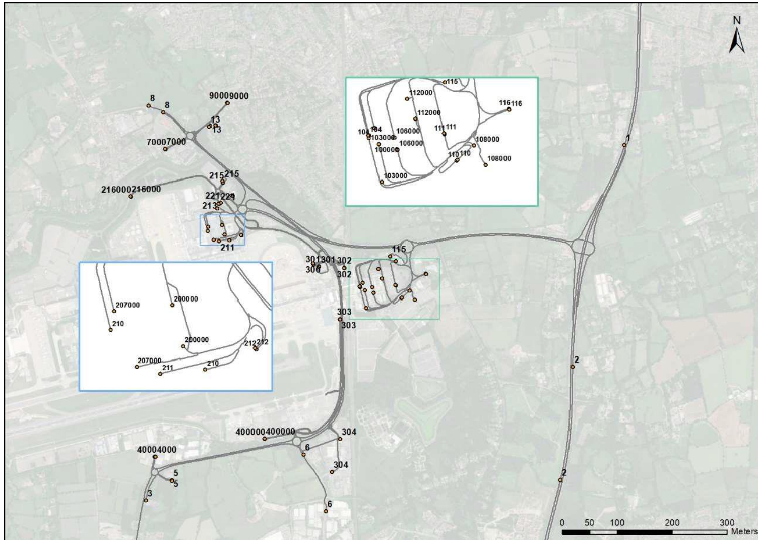
Diagram 5.3.4: Extent of VISSIM local traffic simulation mode
